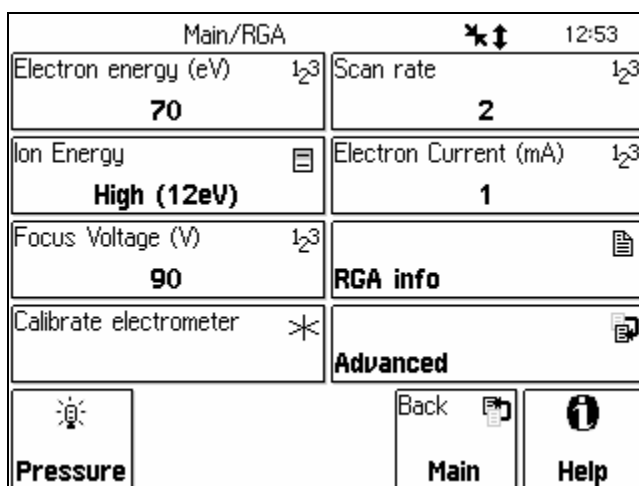
Figure 4. RGA Setup parameters are easily set from the front panel.
