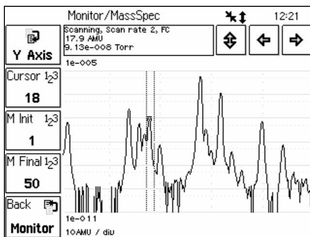
Figure 3. The Mass Spec Display mode of the PPM100 shows complete RGA Mass spectra and includes a cursor for fast peak identification.
