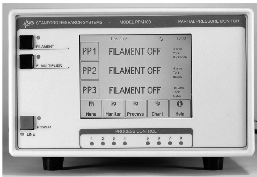
Figure 1. Front panel of the PPM100 controller with its touchscreen/LCD display and RGA control buttons.
